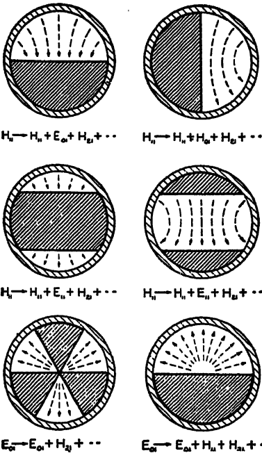
Typical metal baffle plates used as wave converters in circular wave guides. Arrows indicate incident and emergent waves. Formulas give predominant waves passed by each type of baffle.
